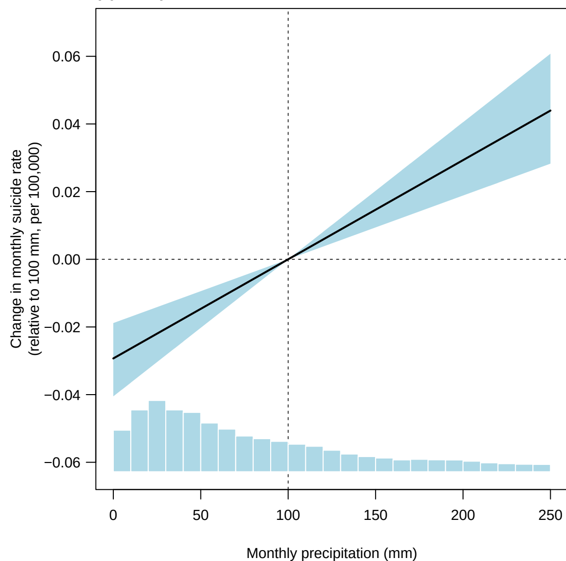
(b) Precipitation
