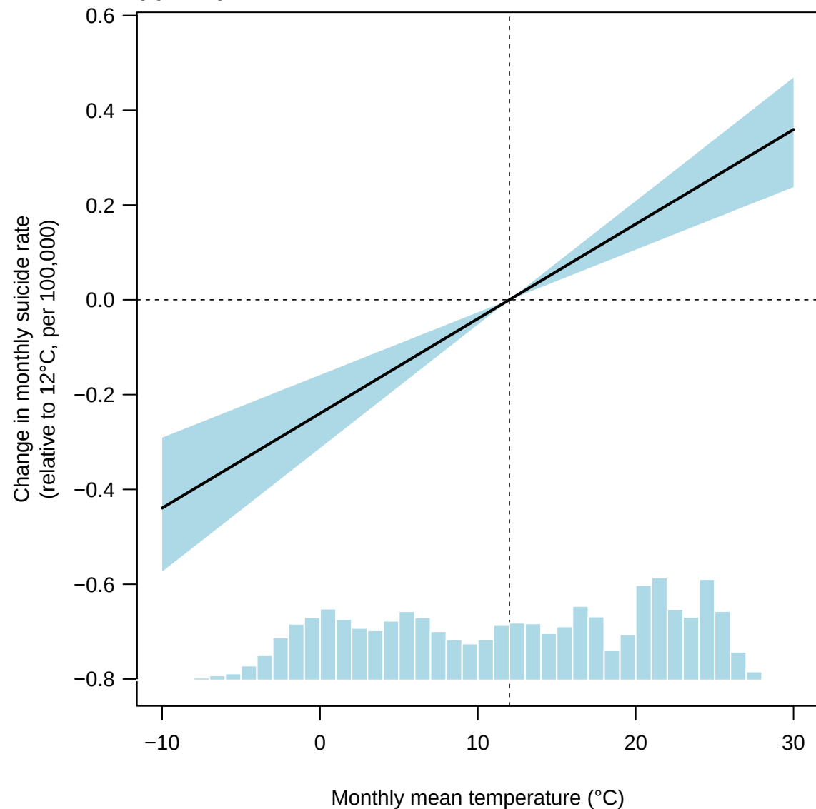
(a) Temperature
